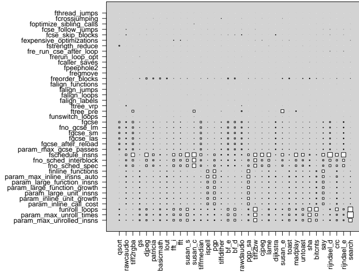
Figure 8: A Hinton diagram showing the optimisations that our model considers most likely to affect performance for each benchmark. The larger the box, the more likely an optimisation affects the performance of the respective program.
